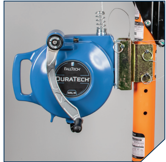
SRL-R shown mounted on Davit System (6050128)
